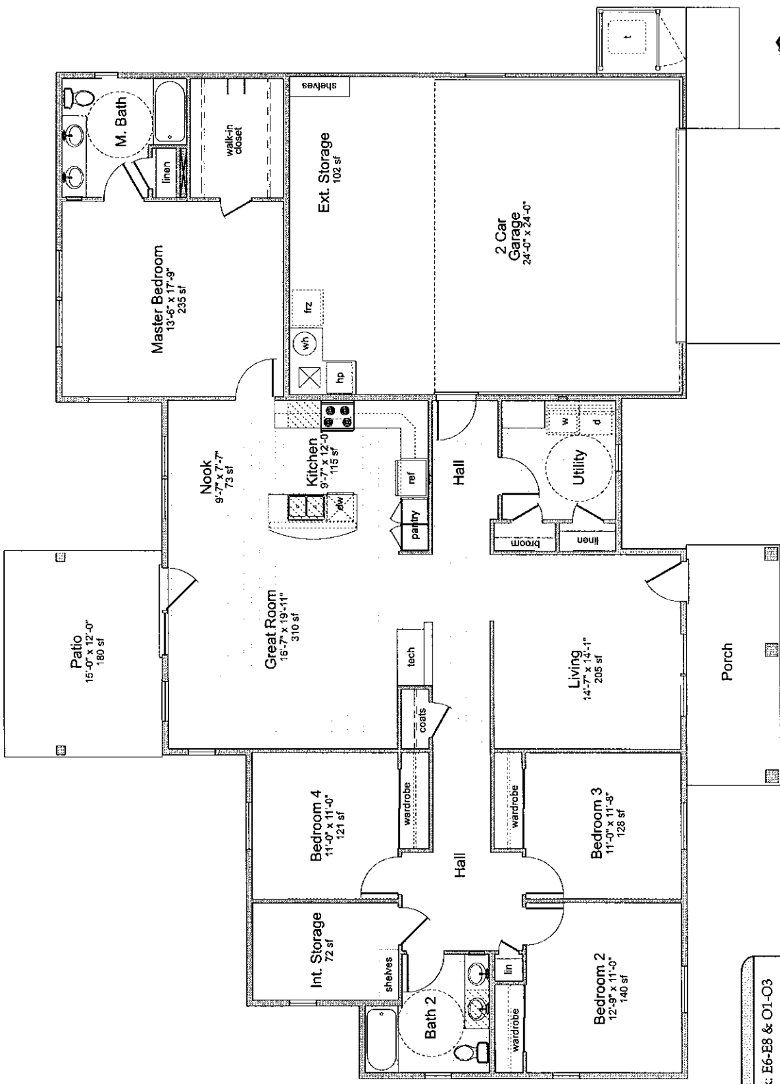
Floor Plan H - Handicap Adaptable (Plan Y Sim.)
